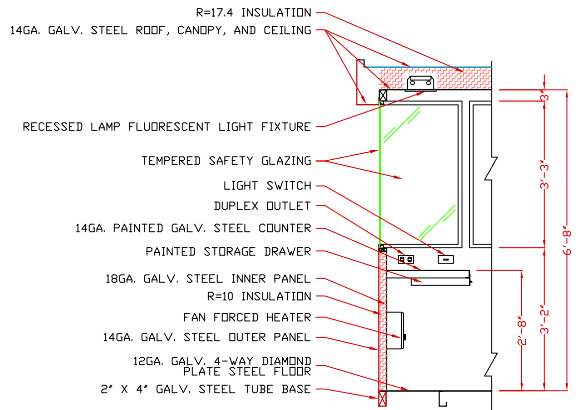
S1 SECTION NO SCALE
