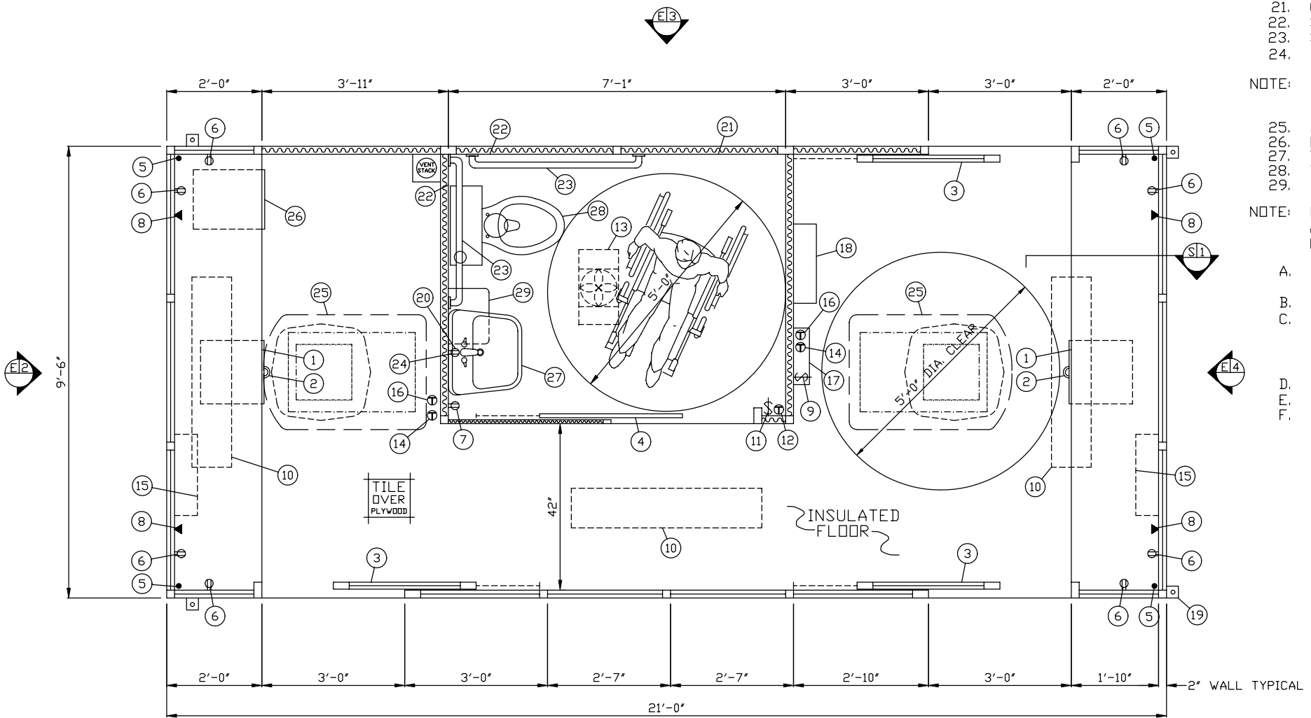
PLAN VIEW
