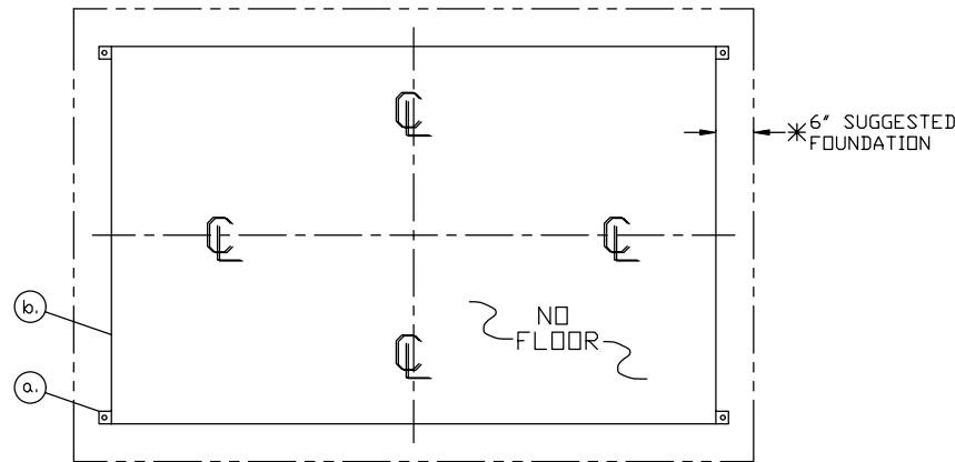
NOTE: PROVIDE 120/240V. 1Ø-3 WIRE SERVICE WITH GROUND. ANCHOR BOLT LAYOUT
