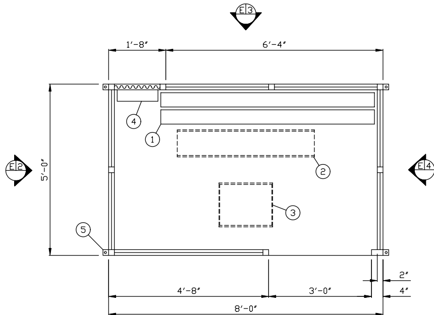
PLAN VIEW
